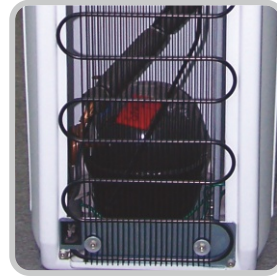
Hermetically sealed reciprocating compressor
