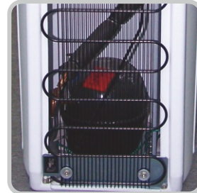
Hermetically sealed reciprocating compressor
